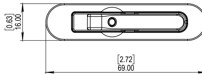
Slot Detail
